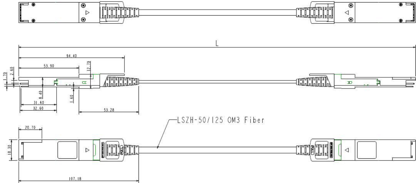
Figure9. Mechanical Specifications
