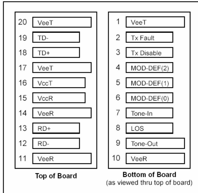
Figure1.Electrical Pin-out Details
