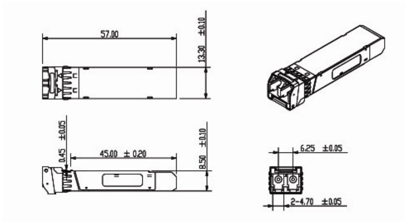
Figure5. Mechanical Dimensions
