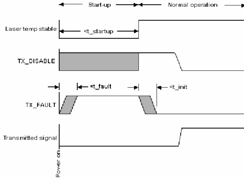
Figure2. Power-on initialisation of DWDM SFP transceiver
